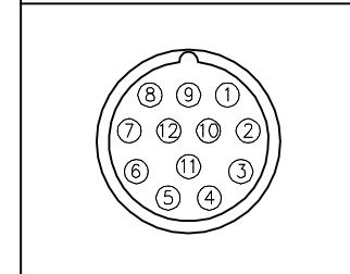
CS 12 PIN-OUT P1
