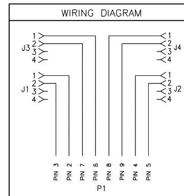
CS 12 PIN-OUT P1
