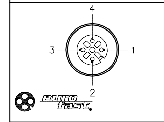
CS 12 PIN-OUT P1
